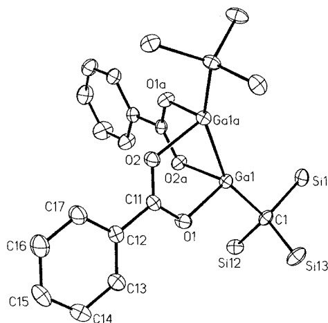
Figure 1. Molecular structure and numbering scheme of compound 7 ; the thermal ellipsoids are drawn at the 40% probability level; methyl groups are omitted for clarity; selected bond lengths (pm) and angles (°): Ga1–Ga1' 240.48(7), Ga1–C1 198.9(2), Ga1–O1 200.6(1), Ga1–O2' 202.9(1), C1–Ga1–Ga1' 156.38(6), O1–Ga1–O2' 91.90(6), O1–Ga1–Ga1' 88.95(4), O2'–Ga1–Ga1' 85.95(4); Ga1' and O2' generated by -x, y, -z + 3/2
