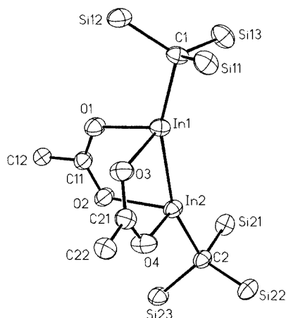
Figure 2. Molecular structure and numbering scheme of compound 8 ; the thermal ellipsoids are drawn at the 40% probability level; methyl groups are omitted for clarity; only the ipso -carbon atoms of the phenyl groups are shown; selected bond lengths (pm) and angles ( ^{\circ} ) [the atoms In3, In4, C3, C4, O5, O6, O7 and O8 belong to the second independent molecule not shown here]: In1–In2 265.44(9), In3–In4 265.38(8), In1–C1 217.2(2), In2–C2 216.7(2), In3–C3 217.0(2), In4–C4 216.9(2), In1–O1 222.8(2), In1–O3 222.8(2), In2–O2 221.6(2), In2–O4 221.1(2), In3–O5 221.4(2), In3–O7 222.8(2), In4–O6 222.4(2), In4–O8 221.3(2); C1–In1–In2 158.74(6), C2–In2–In1 161.07(6), C3–In3–In4 160.43(6), C4–In4–In3 160.50(6), O1–In1–O3 89.93(6), O2–In2–O4 90.77(7), O5–In3–O7 90.38(7), O6–In4–O8 90.79(7), O1–In1–In2 85.13(4), O3–In1–In2 83.58(4), O2–In2–In1 83.99(4), O4–In2–In1 85.53(5), O5–In3–In4 85.15(4), O7–In3–In4 83.41(4), O6–In4–In3 84.01(4), O8–In4–In3 85.63(5).
